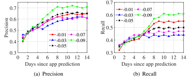
Figure 14: Effect of the decrease rate p .
