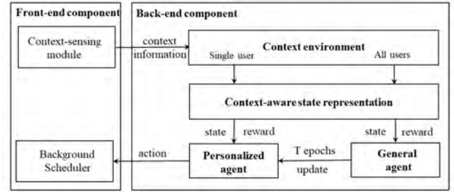
Figure 5: The architecture of app prediction system.
