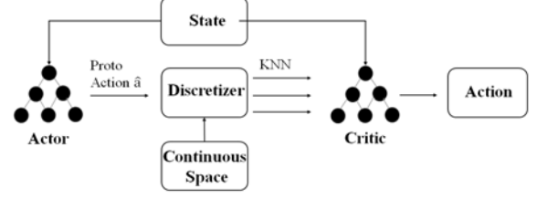
Figure 6: The architecture of the actor-critic agent.
